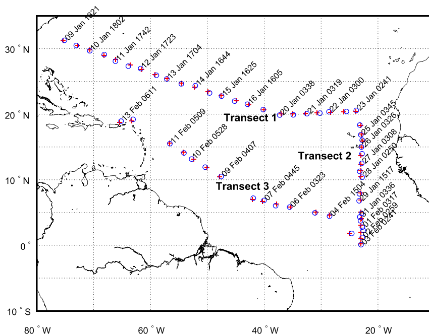
FIG. 1. Dedicated Vaisala RS92 radiosonde launch locations (red plus signs) and nearest collocated (accepted or rejected) NUCAPS footprints (blue circles) for the 2013 AEROSE campaign with three transects defined by northwest–southeast (9–23 Jan), north–south (from 23 Jan to 2 Feb), and southeast–northwest (3–13 Feb).
