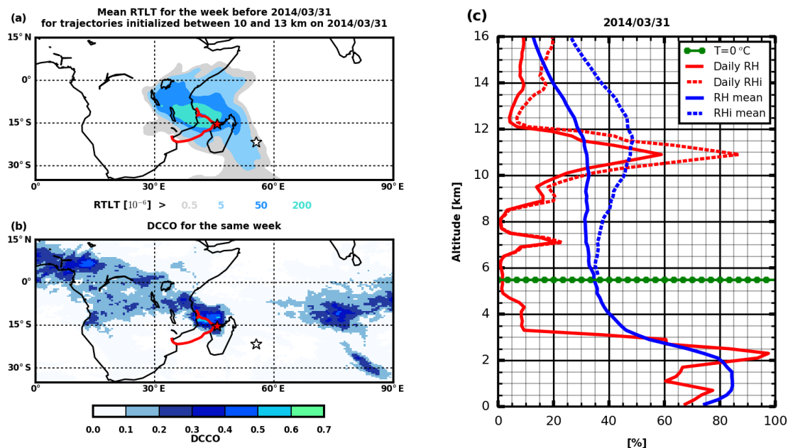
Figure 8. (a) Fraction of residence time below 5 km (RTLT) for air masses initialized in the upper troposphere (10–13 km) over Réunion island on 31 March 2014. (b) Map of DCCO for the week before 31 March 2014. In panels (a) and (b) the best-track data are provided by Météo-France. In the two panels on the left, the red star indicates the position of Tropical Cyclone Hellen on 31 March 2014, and the white star corresponds to the location of Réunion island. (c) RH / RHi profiles on 31 March 2014 (solid and dotted red lines, respectively) and seasonal mean RH / RHi profiles (solid and dotted blue lines, respectively) over austral summers 2014, 2015 and 2016. The dotted green line corresponds to the 0^{\circ}\text{C} isotherm.
